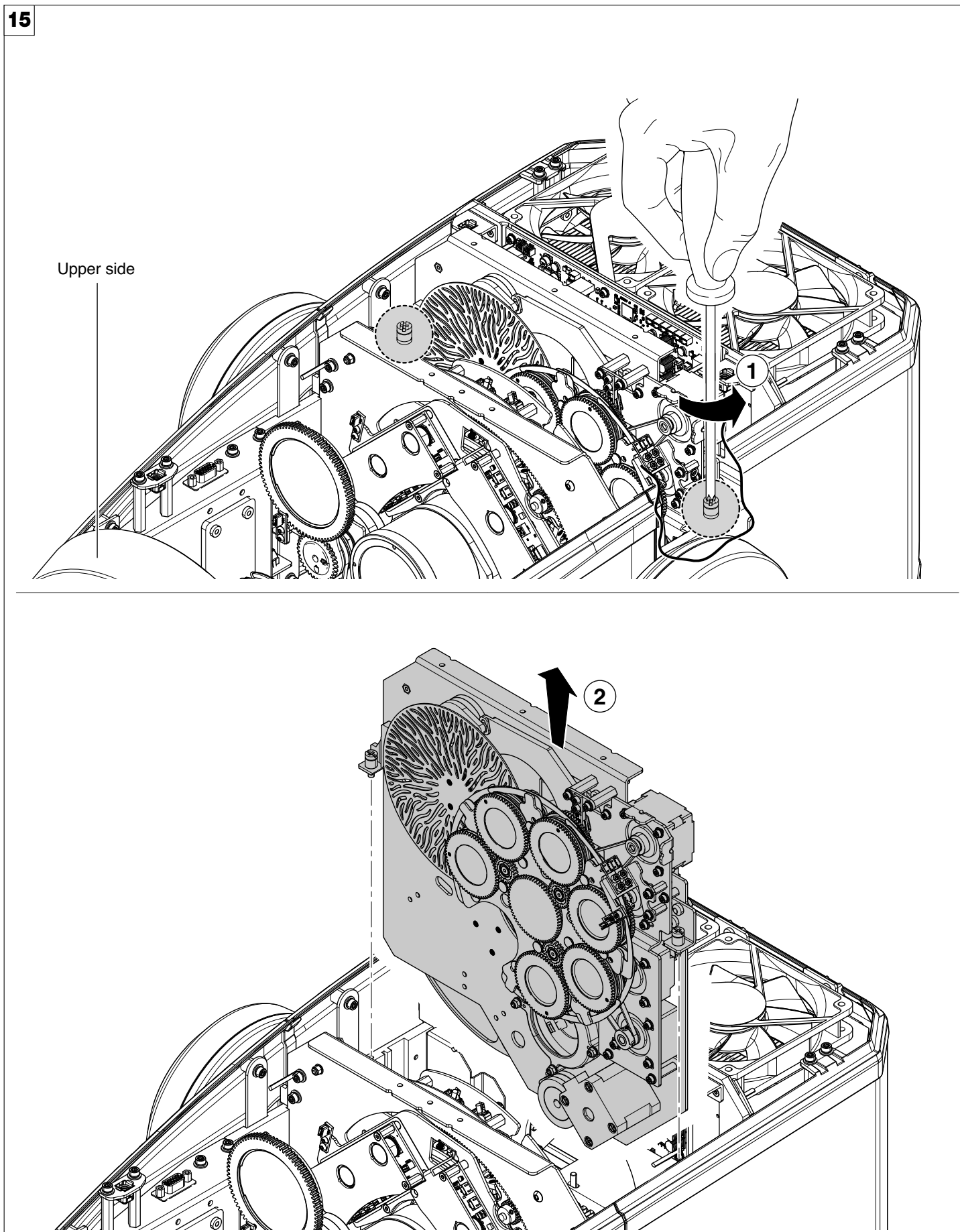
Extraction of the effect modules - Fig. 15.
